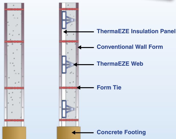
Conventional Poured Concrete Walls
