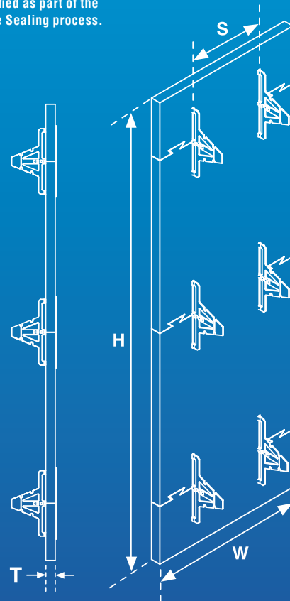
STEP 4: Once the concrete has cured and your forms are removed, the wall is ready for finish board application. Finish materials are easily installed by simply screwing into the exposed face of the ThermaEZE web for a secure hold. It's that easy! Supplemental foam adhesive may also be used for drywall installation.
